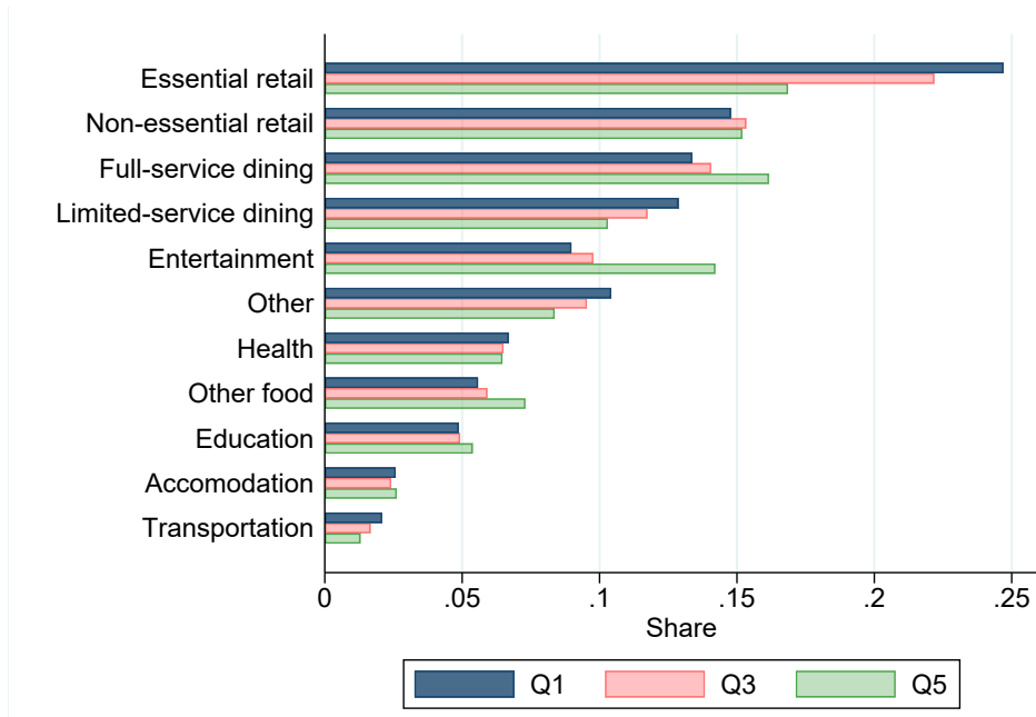
(a) Sector share of visits, by income quintile
