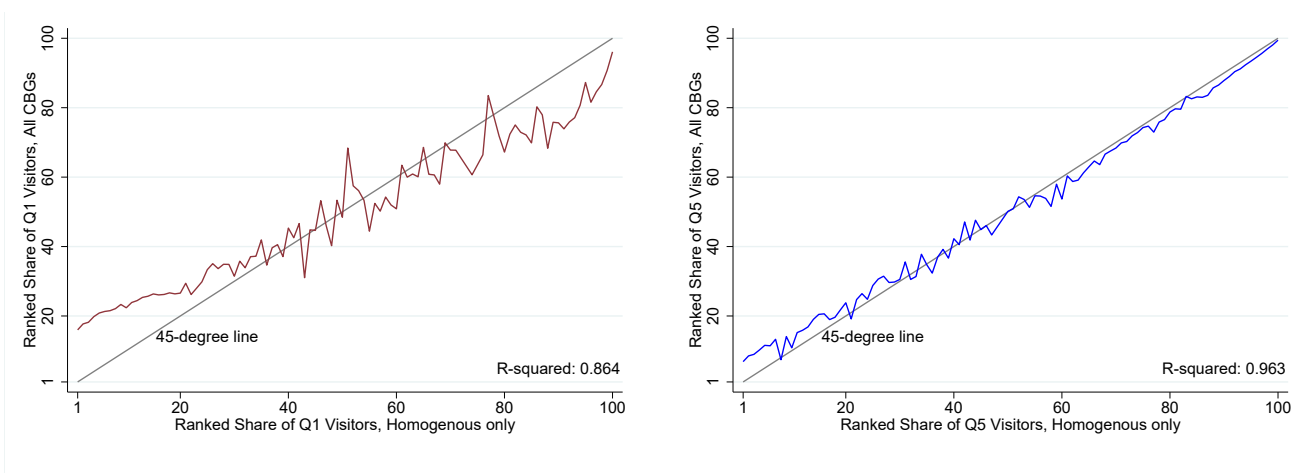
(a) Bottom quintile
