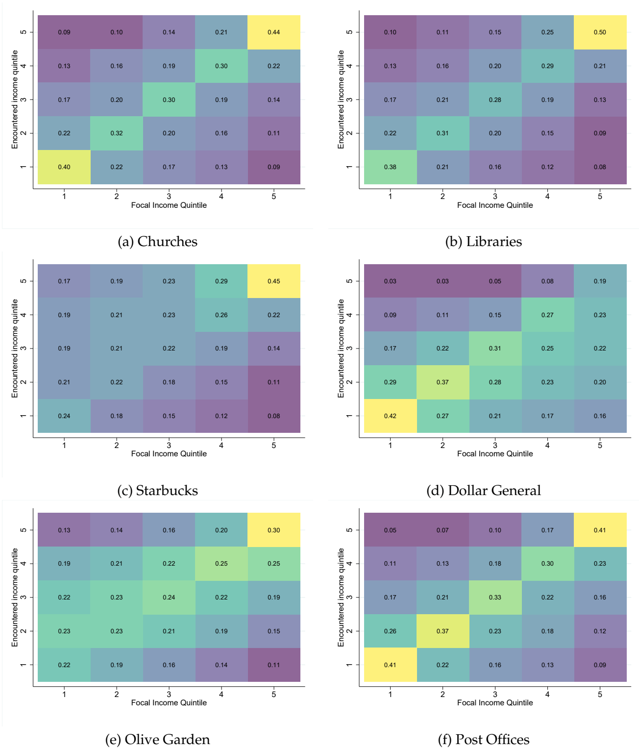
Figure 8: Mixing at different places
