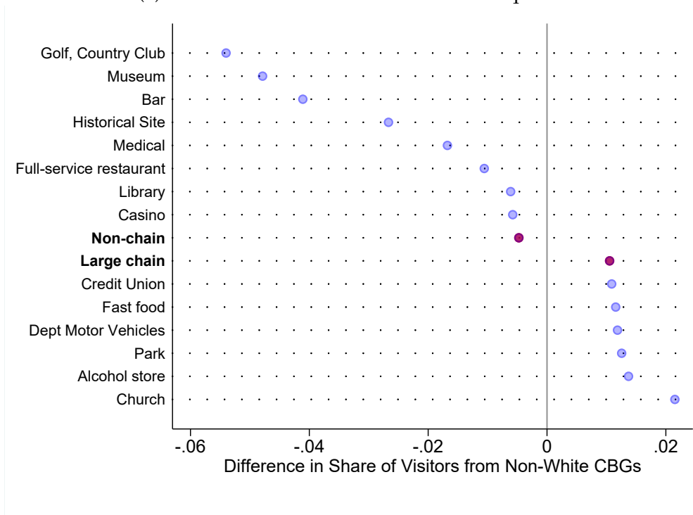
(b) Share of visitors from majority non-white CBGs
